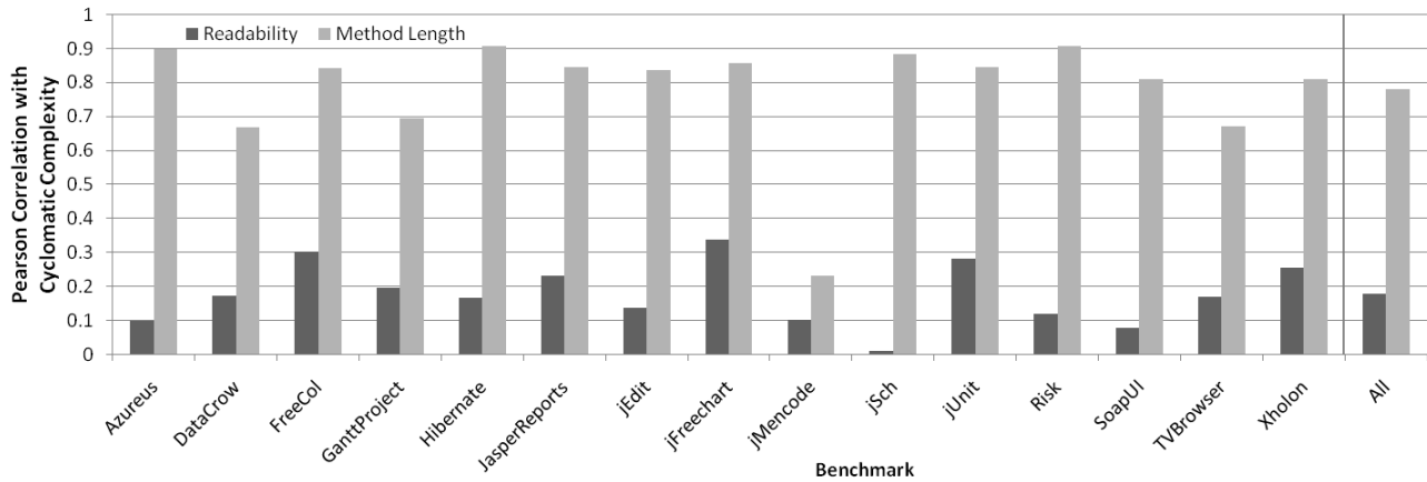
Fig. 13. Pearson Product moment correlation between Cyclomatic complexity and readability as well as between Cyclomatic complexity and method length (number of statements in the method). Readability is at most weakly correlated with complexity in an absolute sense. In a relative sense, compared to method length, readability is effectively uncorrelated with complexity. These results imply that readability captures an aspect of code that is not well modeled by a traditional complexity measure.
