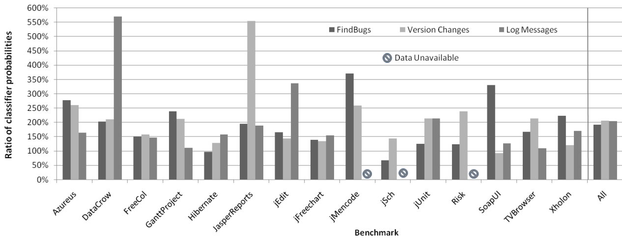
Fig. 12. Mean ratio of the classifier probabilities (predicting ‘less readable’) assigned to functions that contained a FindBugs defect, that will change in the next version, or that had a defect reported in a version control log. For example, FreeCol functions with FindBug errors were assigned a probability of ‘less readable’ that was nearly 150% greater on average than the probabilities assigned to functions without such defects.
