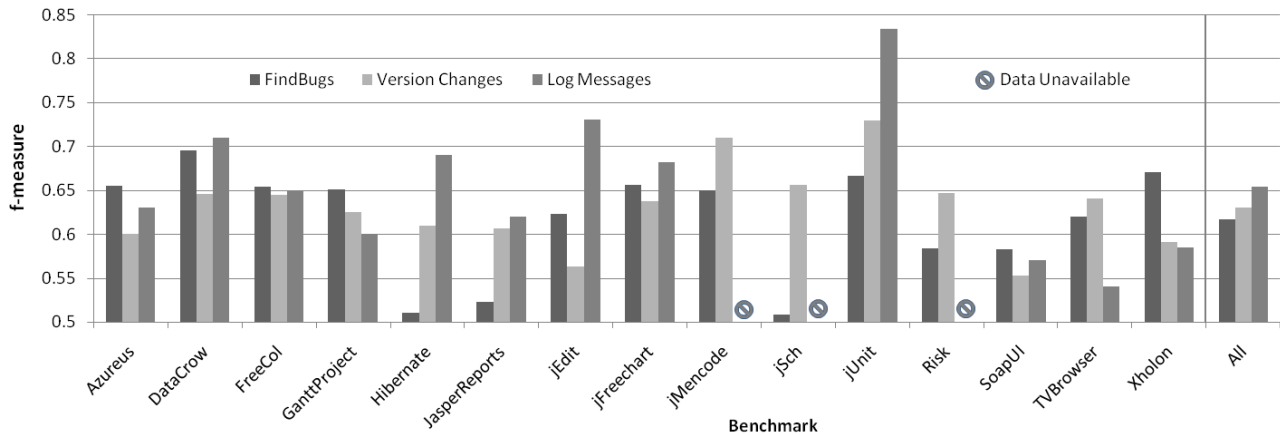
Fig. 11. f-measure for using readability to predict functions that: show a FindBugs defect, have change between releases, and have a defect referenced in a version control log message. For log messages, “Data Unavailable” indicates that not enough version control information was available to conduct the experiment on that benchmark.
