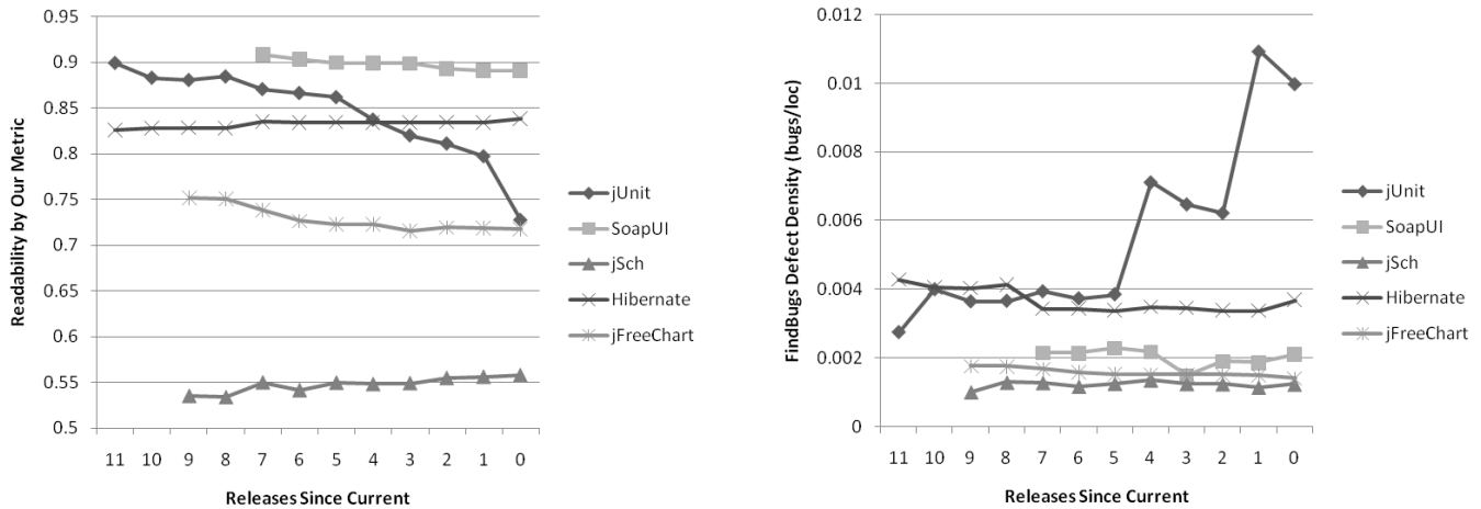
Fig. 14. The left graph shows the average readability metric of all functions in a project as a function of project lifetime. The right graph shows the FindBugs defect density in a project as a function of project lifetime for the same projects and releases. Note that the projects with flat readabilities have corresponding flat defect densities, while jUnit (described in text) becomes significantly less readable and significantly more buggy starting at release 5.
