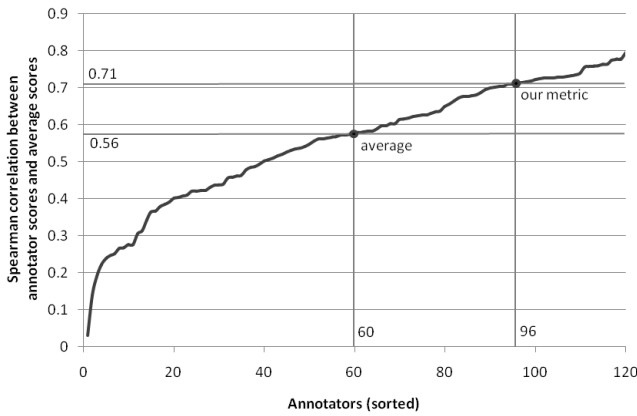
Fig. 7. Inter-annotator agreement. For each annotator (in sorted order), the value of Spearman's \rho between the annotator's judgments and the average judgments of all the annotators (the model that we attempt to predict). Also plotted is Spearman's \rho for our metric as compared to the average of the annotators.
